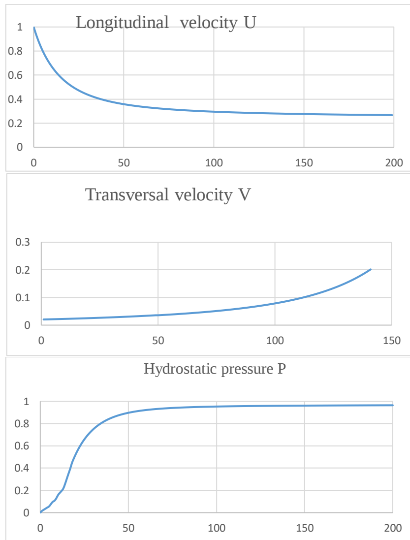
Figure 2. Scholars based on the transverse, longitudinal velocity of the stream and the number of pressure obtained by the channel
